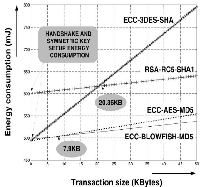
Figure 2. The impact of cipher suite selection on energy consumption during the SSL handshake and record stages.
